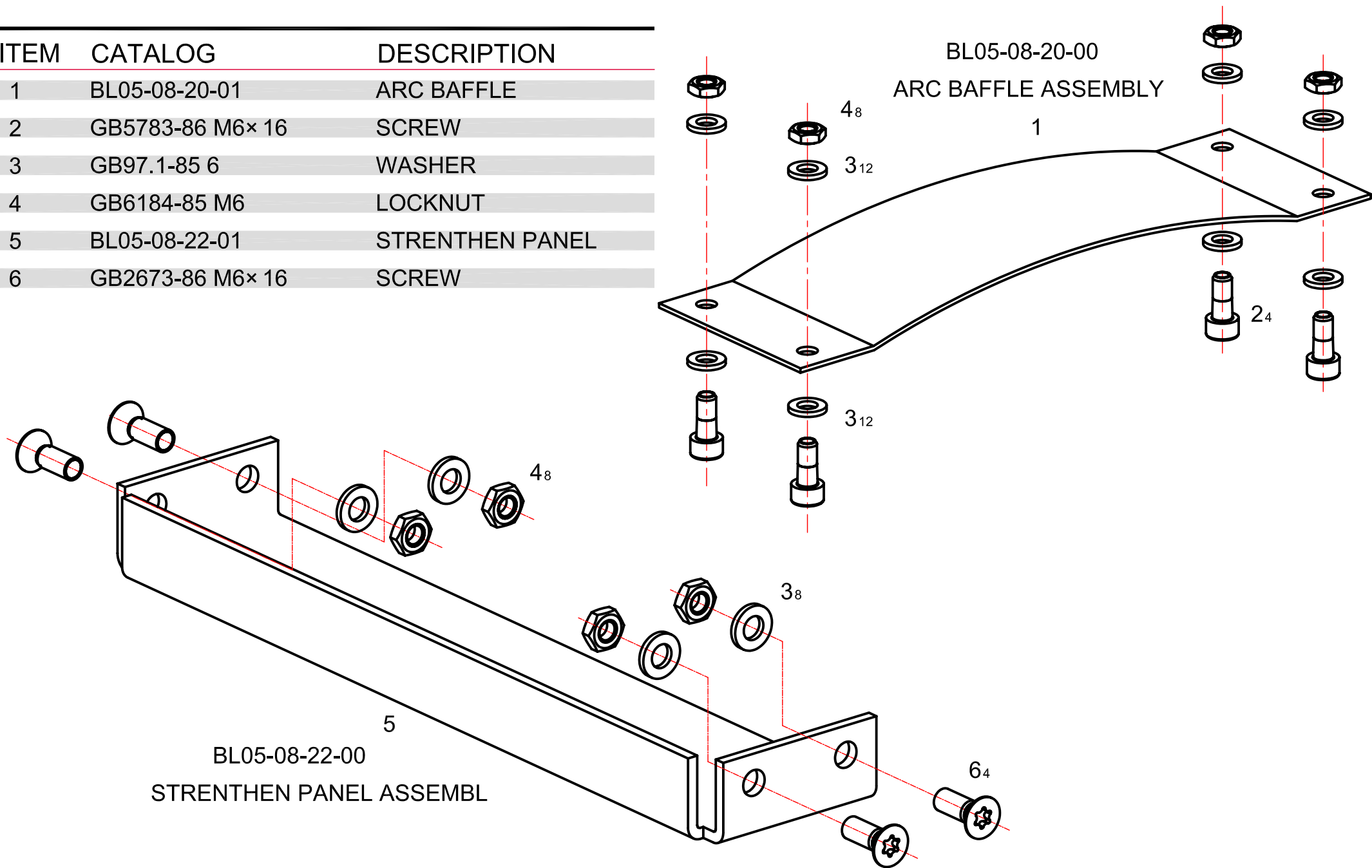
ARC BAFFLE ASSEMBLY BL05-08-20-00 & STRENGTHEN PANEL ASSEMBLY BL05-08-22-00
