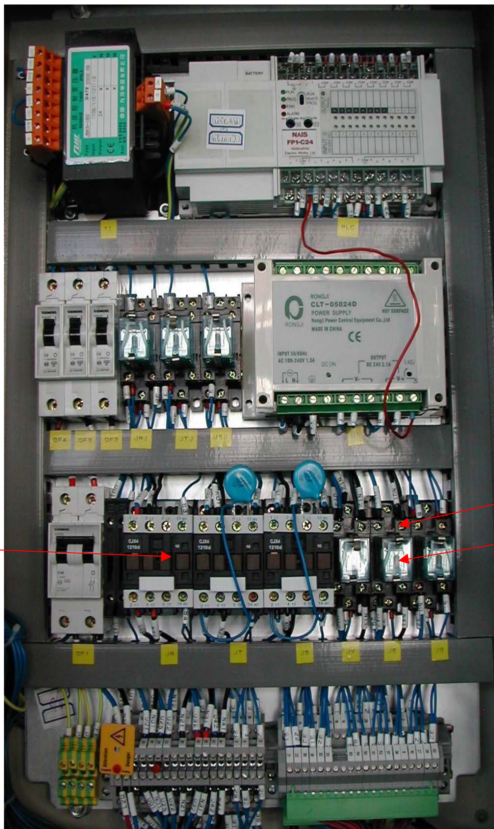
MC2 Pinsetter Control Box Without Pit Light Control
