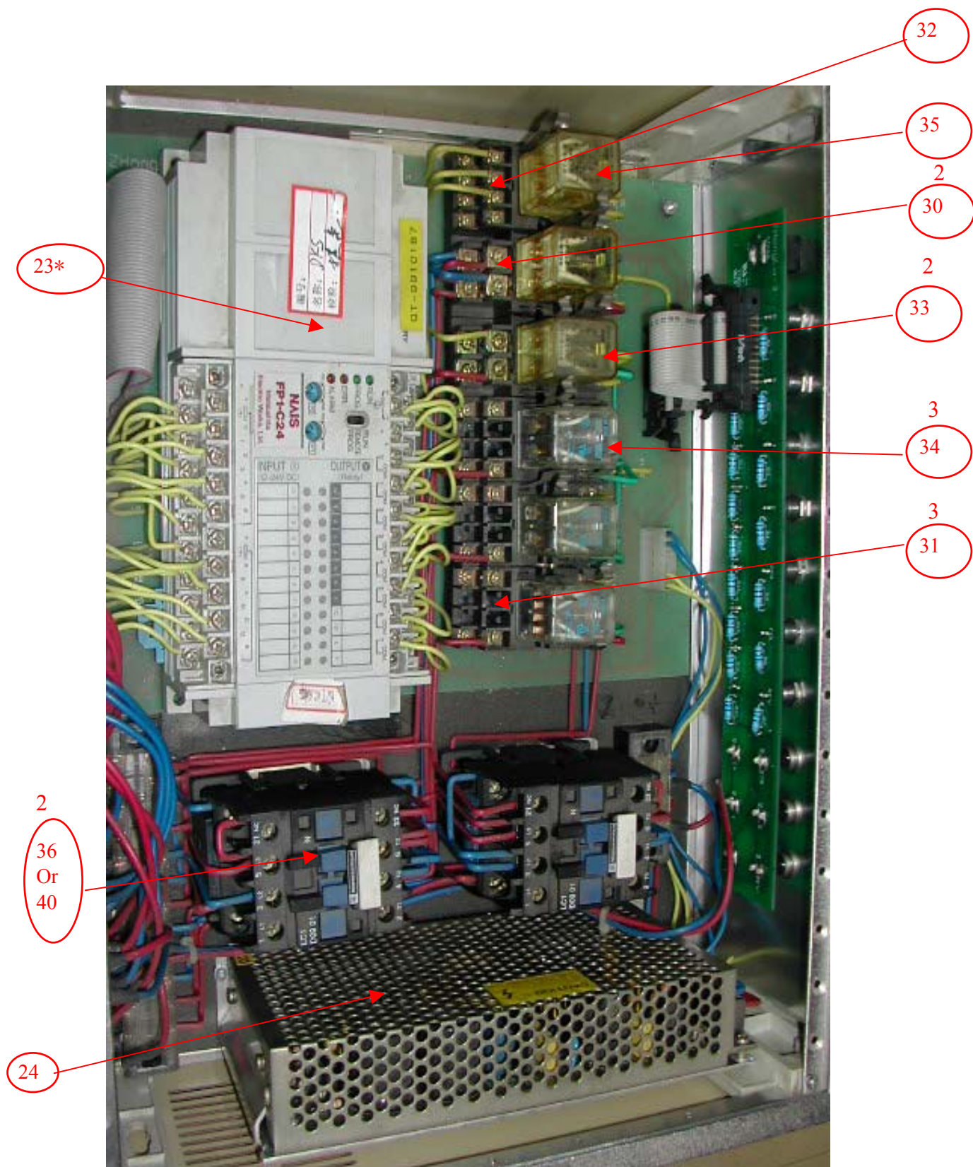
QBKII Control Box
