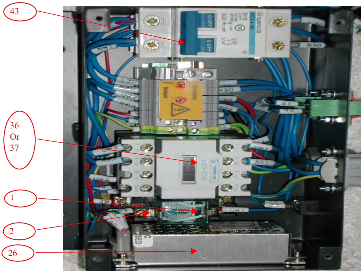
Fastrack Control Box
