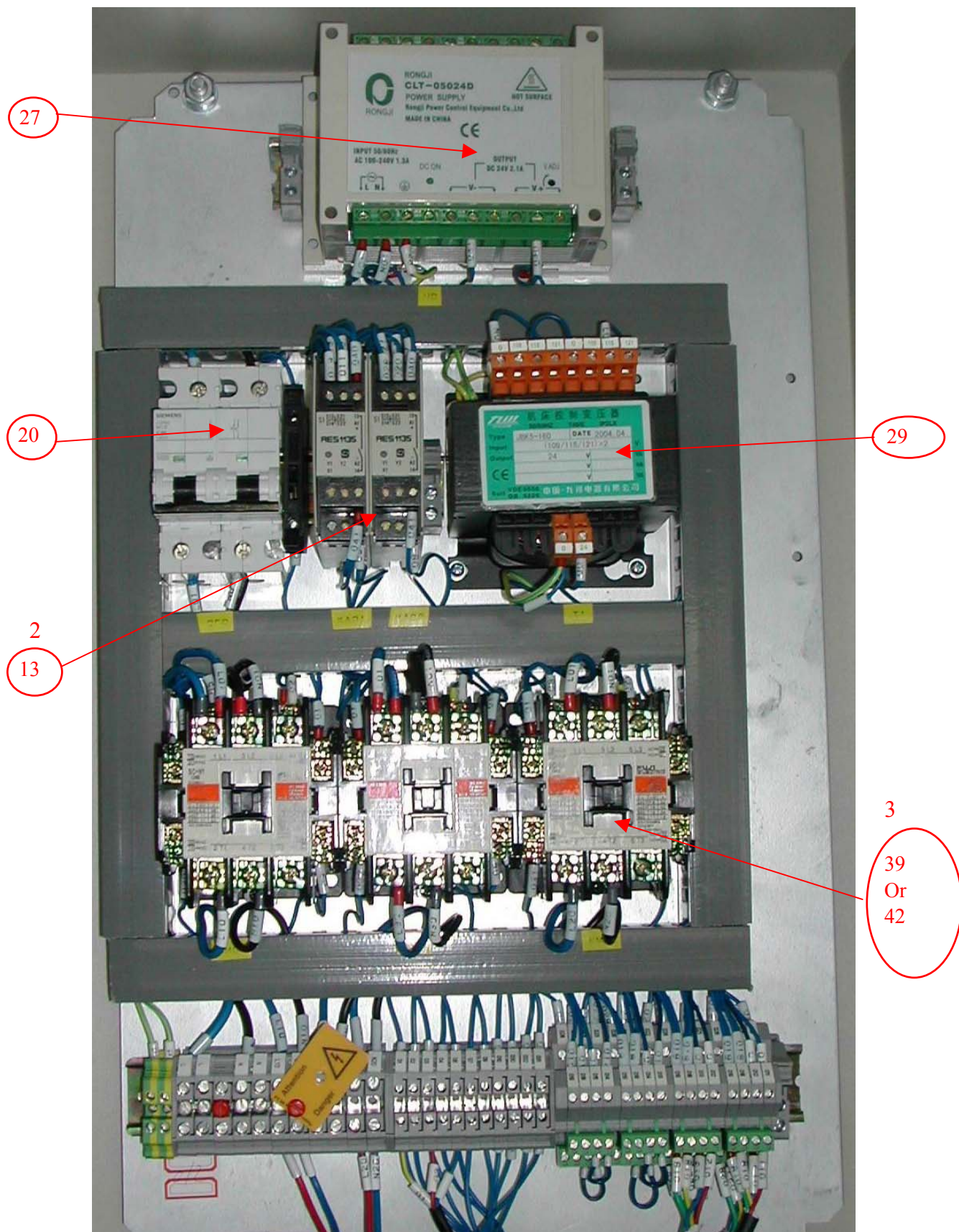
MC2 High Voltage Manage Box
